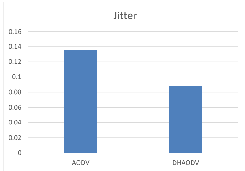
Figure 4.Jitter Output
