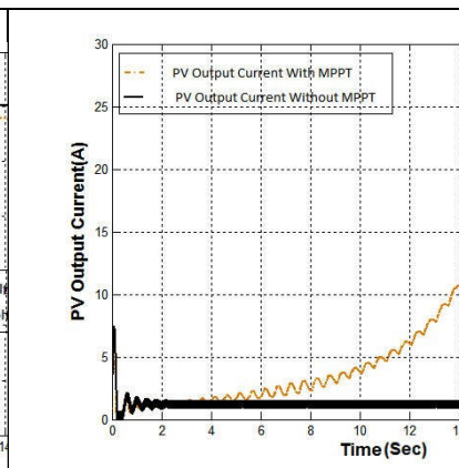
Figure 12 Output Current for the solar irradiance (1000 w/m 2 ) in hybrid MPPT technique
