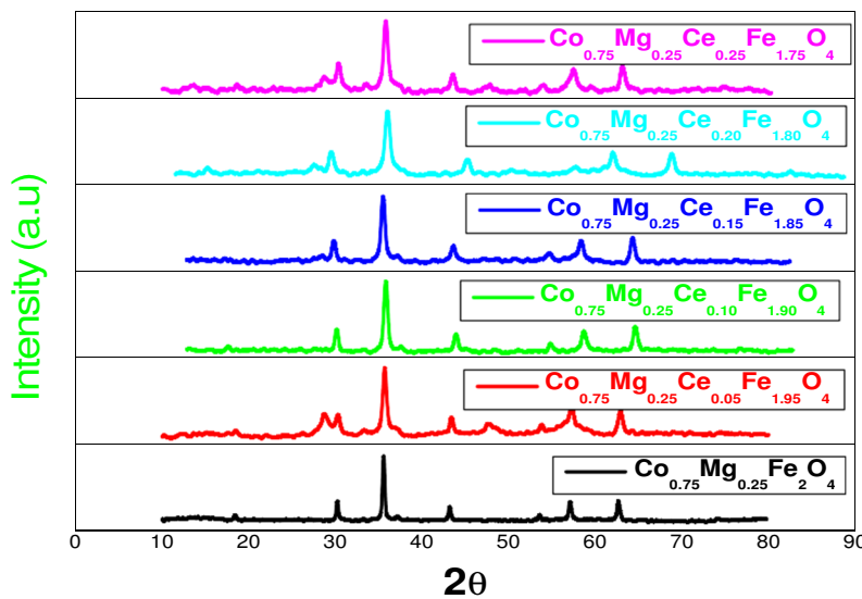
Fig 1.1 XRD pattern of Co-Mg-Ce nano ferrites
