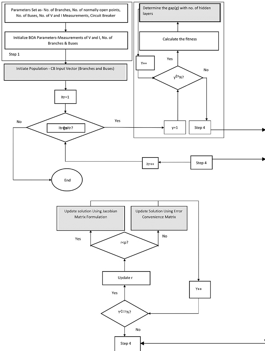
Fig.3 Flowchart of the general BOA steps
