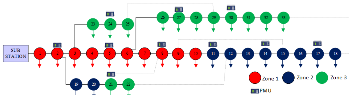
Fig 5. Bus classification scheme
