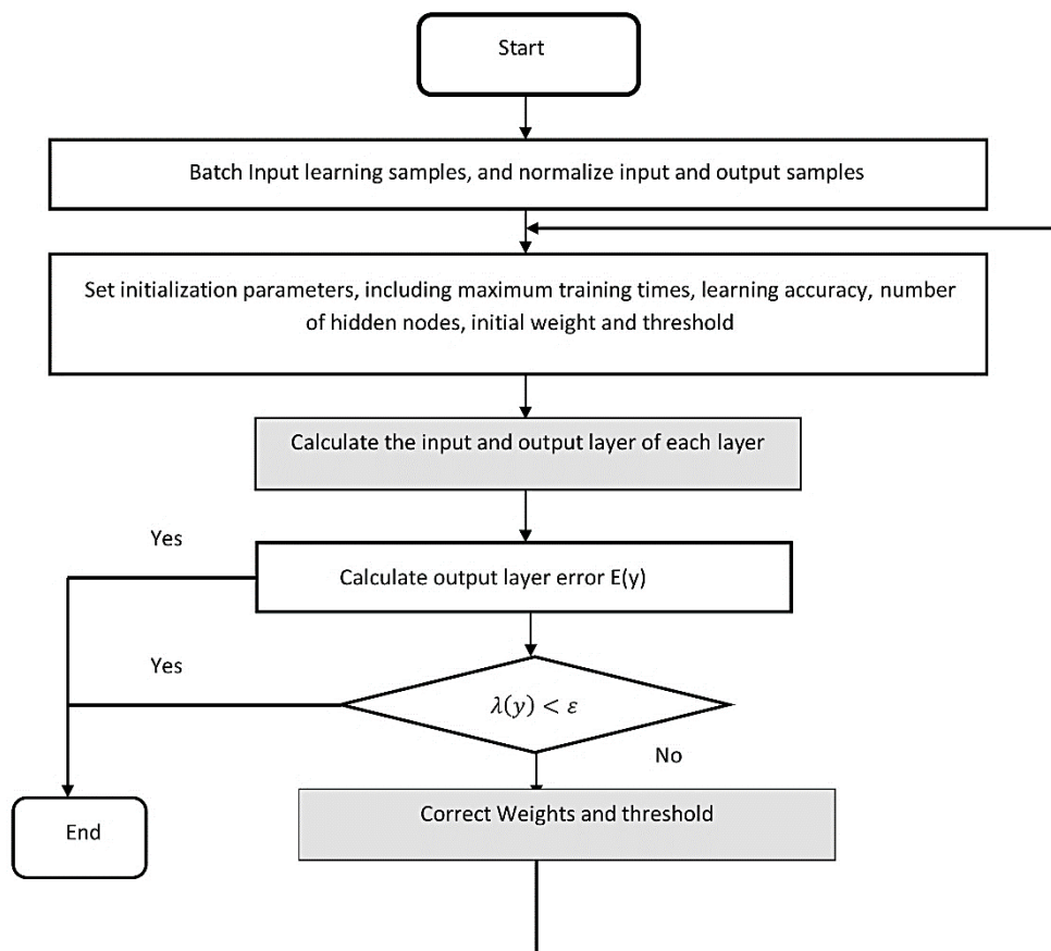
Fig.4 Machine Learning Flowchart
