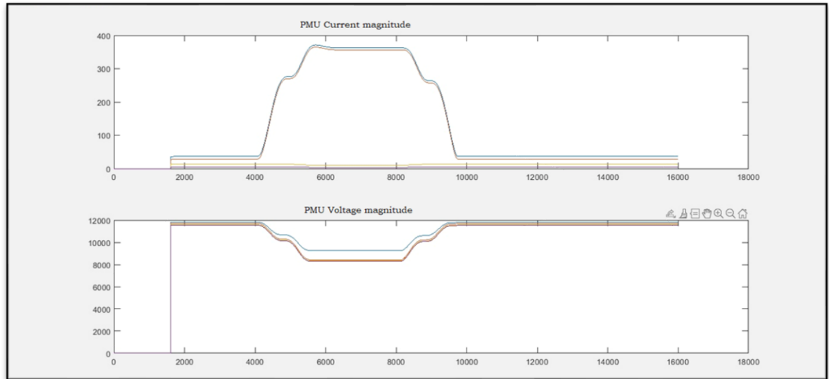
Fig.8. PMU Voltage and Current for LG Fault
