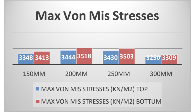
Graph.4: Max von mis Stresses on Deck Slab of 10m Span with varying thickness
