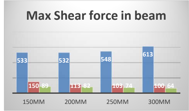
Graph.10: Maximum Shear force on Beam of 10m Span with varying thickness
