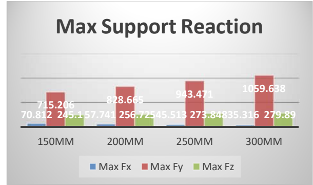
Graph.18: Maximum Support reaction of 18m Span with varying thickness
