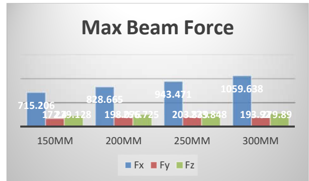
Graph.12: Maximum Shear force on Beam of 18m Span with varying thickness
