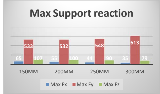
Graph.16: Maximum Support reaction of 10m Span with varying thickness
