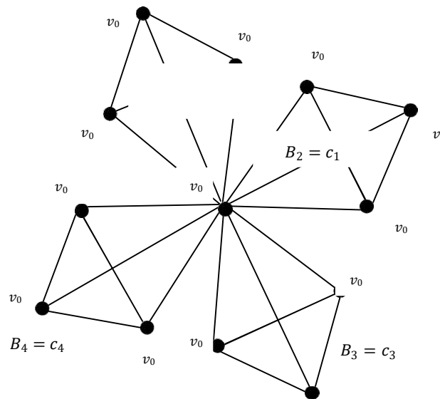
Fig 4: Windmill Wd(4,4)
